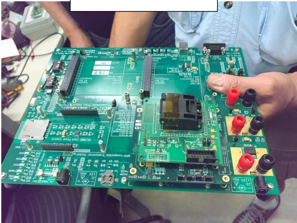
CubeSat Hardware
